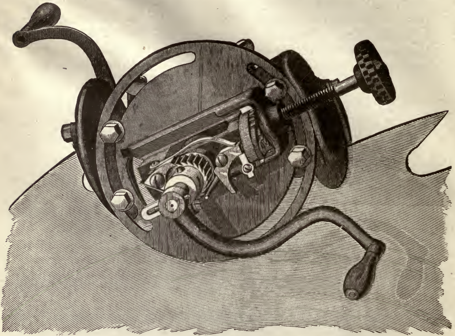
FIG. 1. ADJUSTED TO GUM CIRCULAR SAWS.
