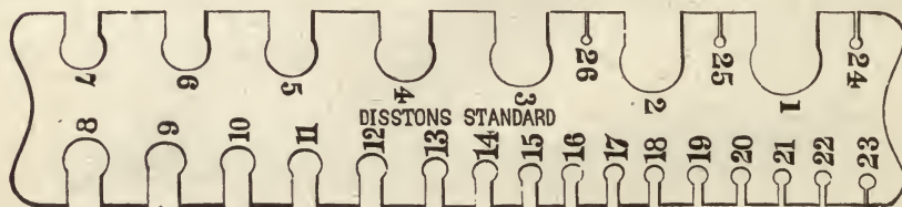
No. 1. Small Gauge, 1 to 26
