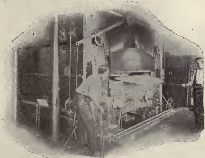
Tempering Circular Saws.
