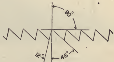
CROSS-CUT TEETH \frac{1}{4} " SPACE.
